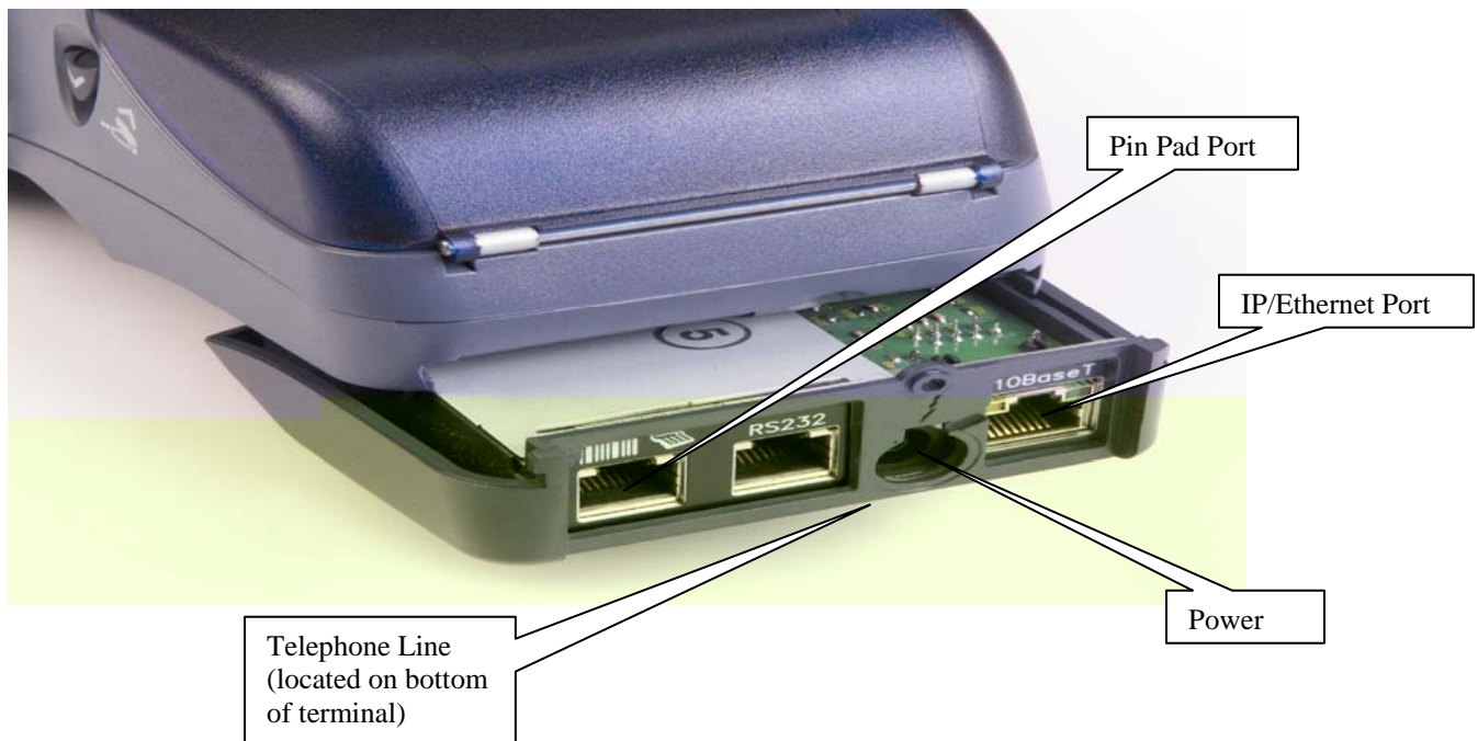
Omni 3750 Dual Comm Terminal Ports
